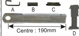
OMC-P-806 CONNECTOR LINK 190MM 1661, 1681, 1761, 1781 F283.137.01
